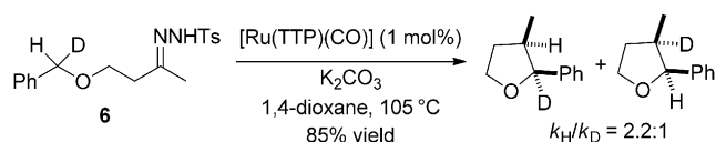
Scheme 5. KIE for the [Ru(TPP)(CO)]-catalyzed cyclization of 6 .
