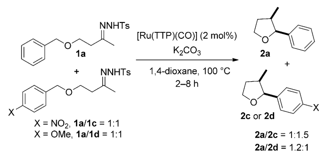
Scheme 6. Competition experiments: [Ru(TPP)(CO)]-catalyzed cyclization of 1a and 1c/1d .
